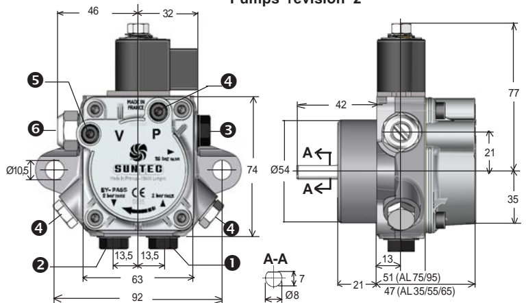
Pumps revision 2
